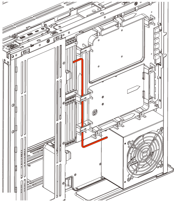
1 24-pin cable channel
