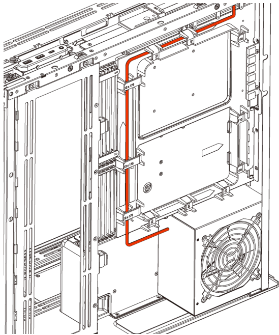
2 4+4-pin cable channel
